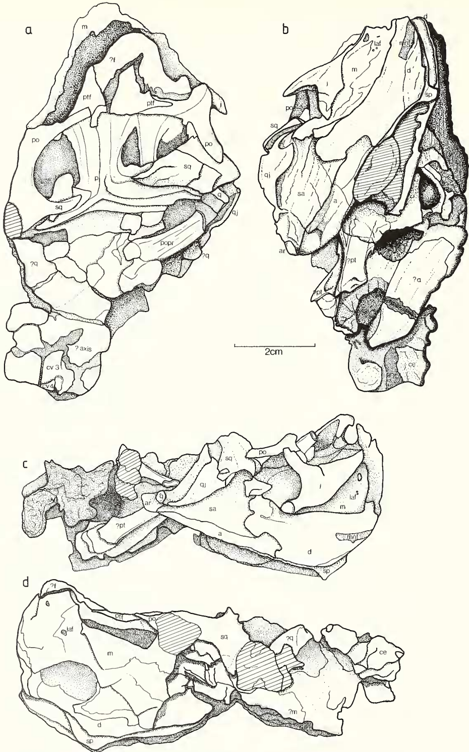
TEXT-FIG. 4. Skull of juvenile Scaphonyx fischeri (MCZ 1664) in dorsal (a), ventral (b), right lateral (c), and left lateral (d) views. Abbreviations are listed in the Appendix.
